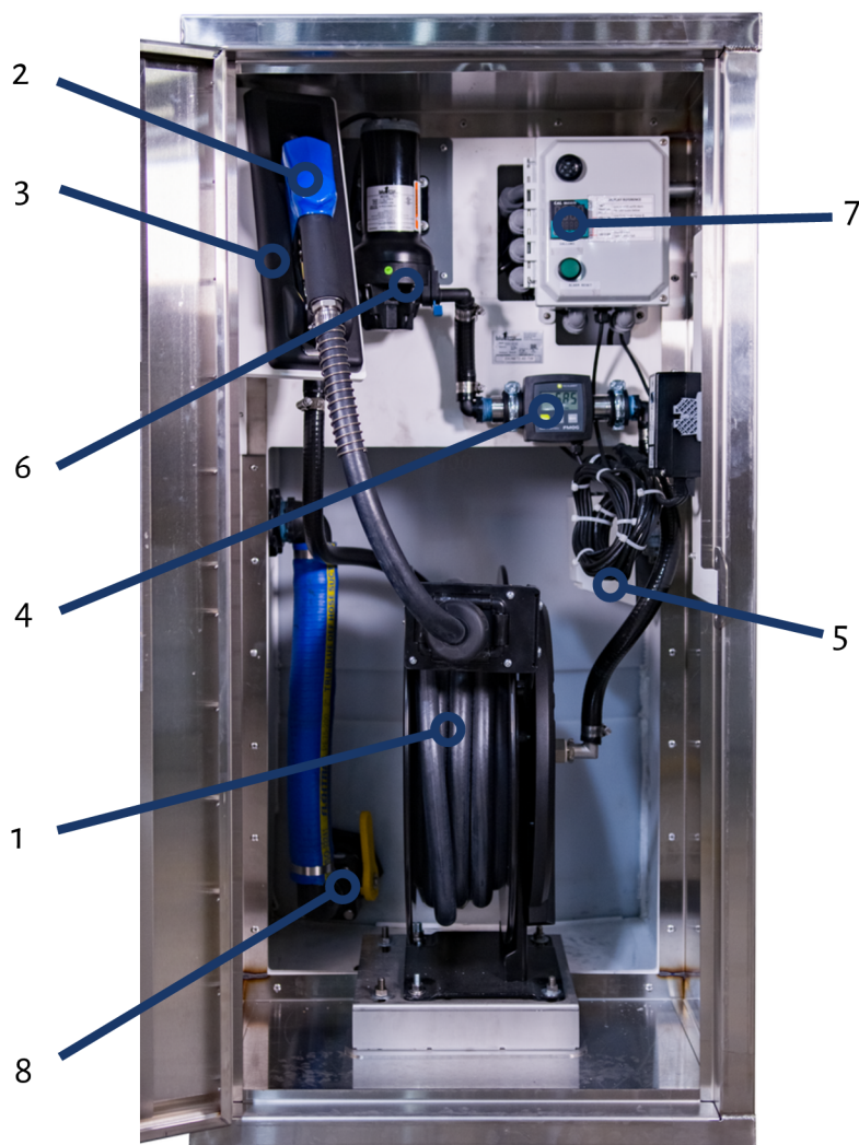
Cabinet with Pulse Meter
