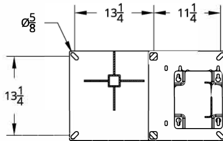
SECTION A - A ANCHOR PATTERN
